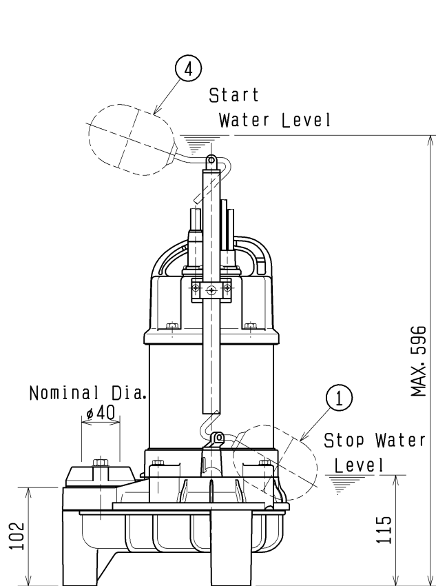
No. 1 PUMP
